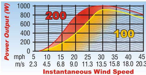
Performance Curves
